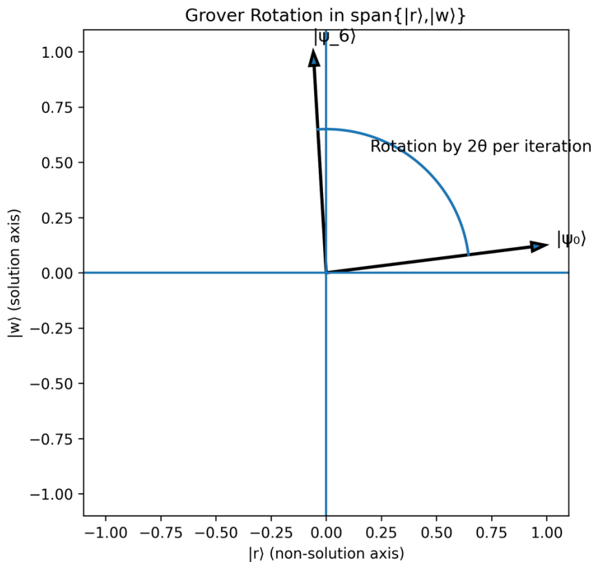
Figure 4. Geometric Rotation in the Two-Dimensional Invariant Subspace
