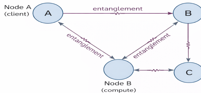
Figure 6. Conceptual Distributed Grover Search over a Quantum Network.
