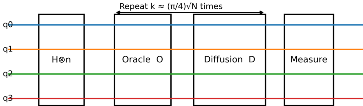
Figure 5. Grover Algorithm Circuit Structure
